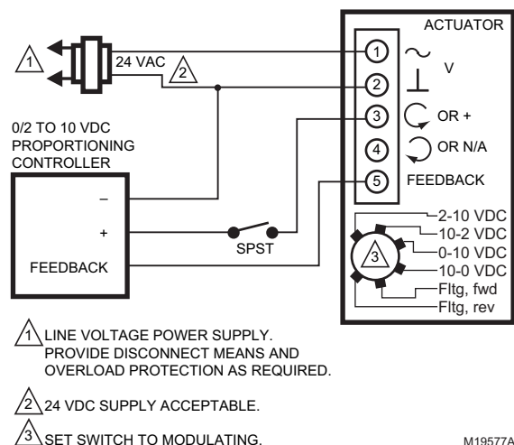
Fig. 36. Override to full closed (Modulating mode setting)
