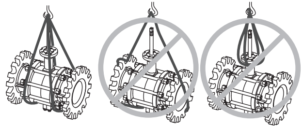
Fig. 6. Proper hoisting of VBF Valves
