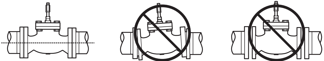
Fig. 8. Basic pipe orientation
