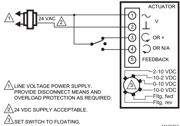
Fig. 23. Wiring for Floating Control (Floating mode setting)
