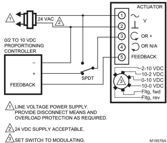
Fig. 24. Override to full open (Modulating mode setting)
