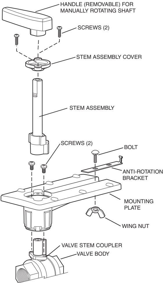
Fig. 16. Valve assembly, exploded view
